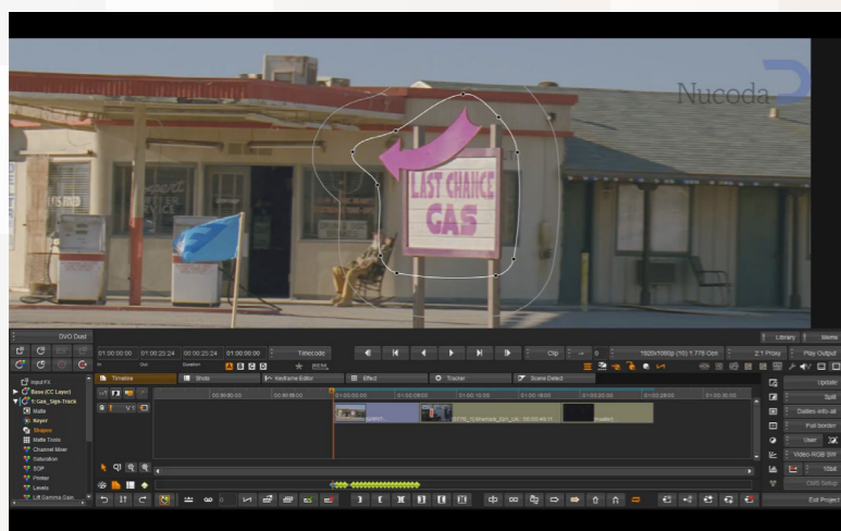
Deformation Tracker
